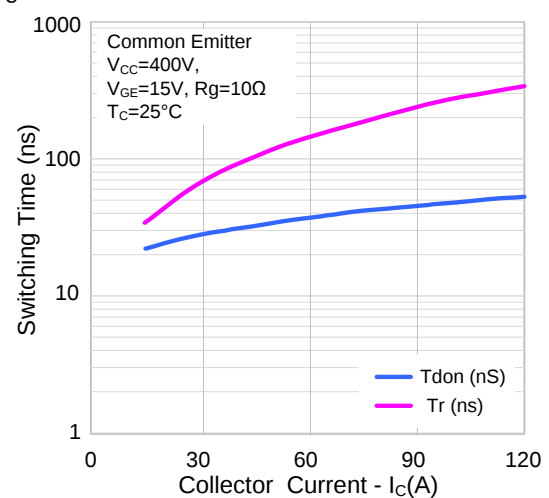
Figure 12. Turn-on Characteristic vs. Collector Current
