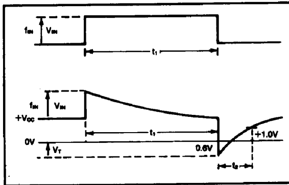
FIGURE 2. F/V Input Waveforms.
