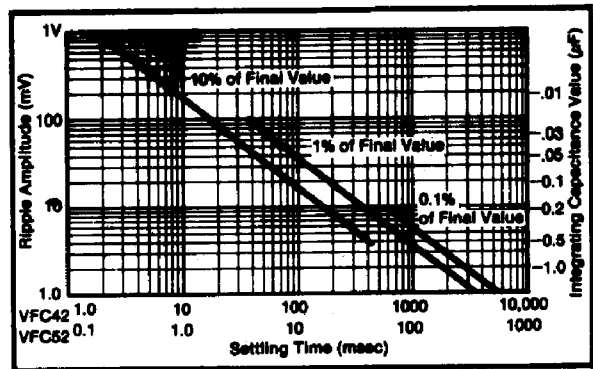
FIGURE 3. F/V Mode Output Settling Time vs. Ripple Voltage Amplitude for Full Scale Frequency Change.
