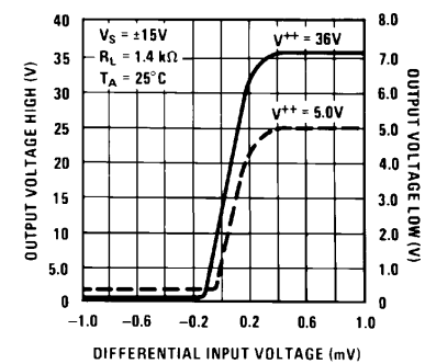
Transfer Function
