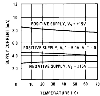
Supply Currents
