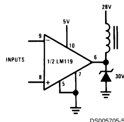
Relay Driver
