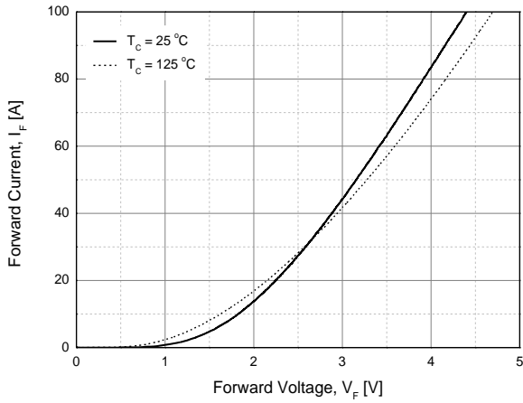
Fig. 18 Conduction characteristics
